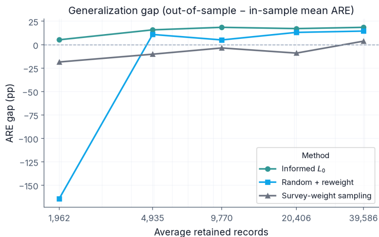
Figure 3: Generalization gap: out-of-sample minus in-sample mean ARE against the average retained-record count, for the three methods. A gap near zero means the retained sample reproduces the held-out families about as well as the families it was fit to; a positive gap measures the cost of generalization, and a negative gap (random + reweight at the smallest budget) marks a case where the in-sample mean is as inflated as the out-of-sample mean. Each line is the mean over three seeds.
