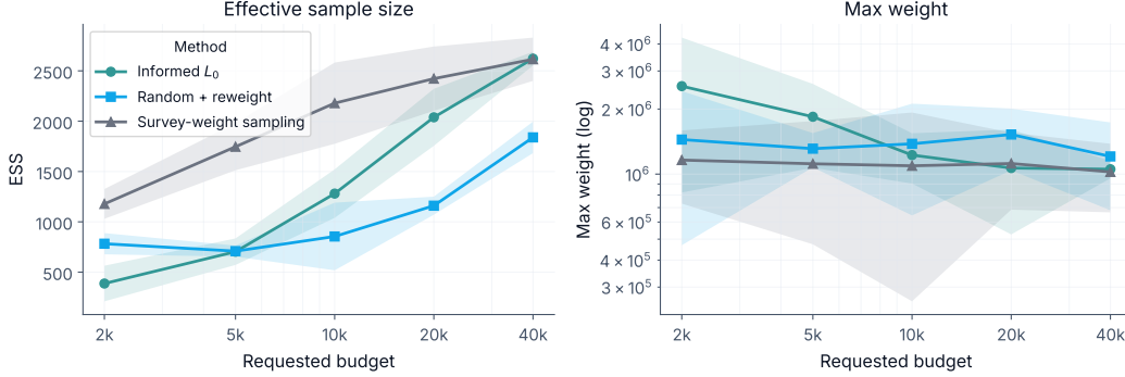
Usability: effective sample size and weight concentration
