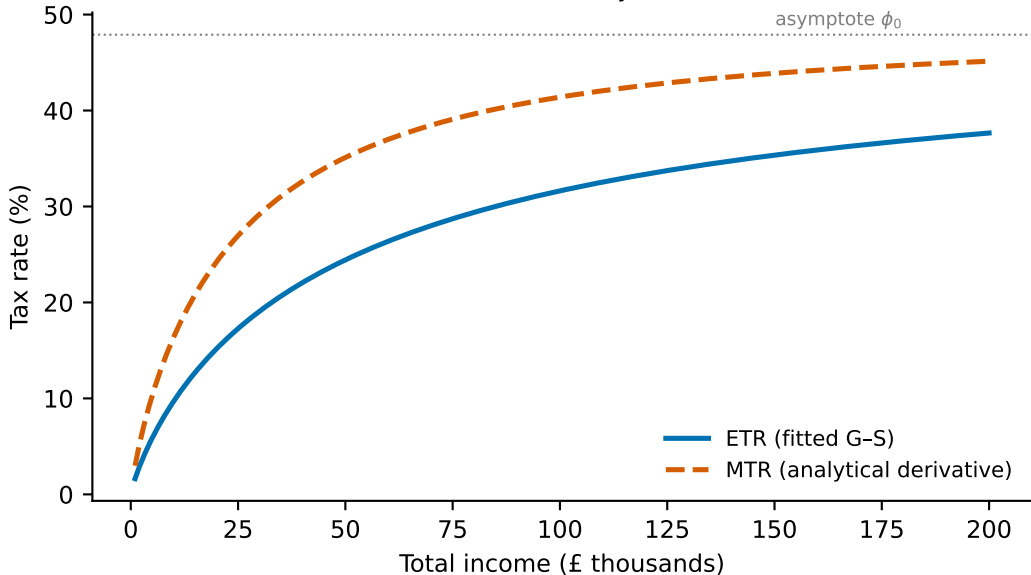
Gouveia-Strauss schedule: mutually consistent ETR and MTR
