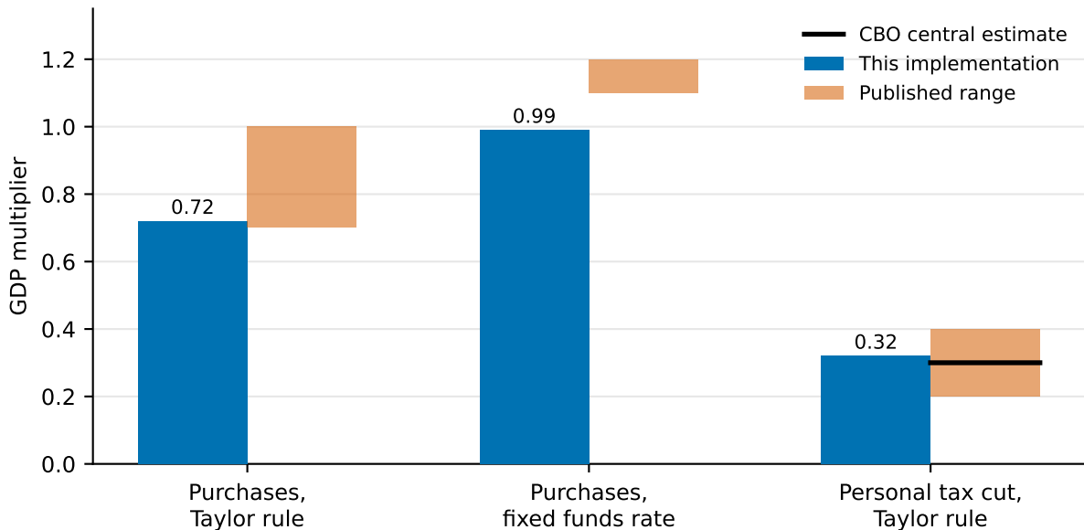
Fiscal multipliers: this implementation vs published benchmarks (purchases: yr 1 Taylor / yr 2 fixed rate; tax cut: yr 2)
