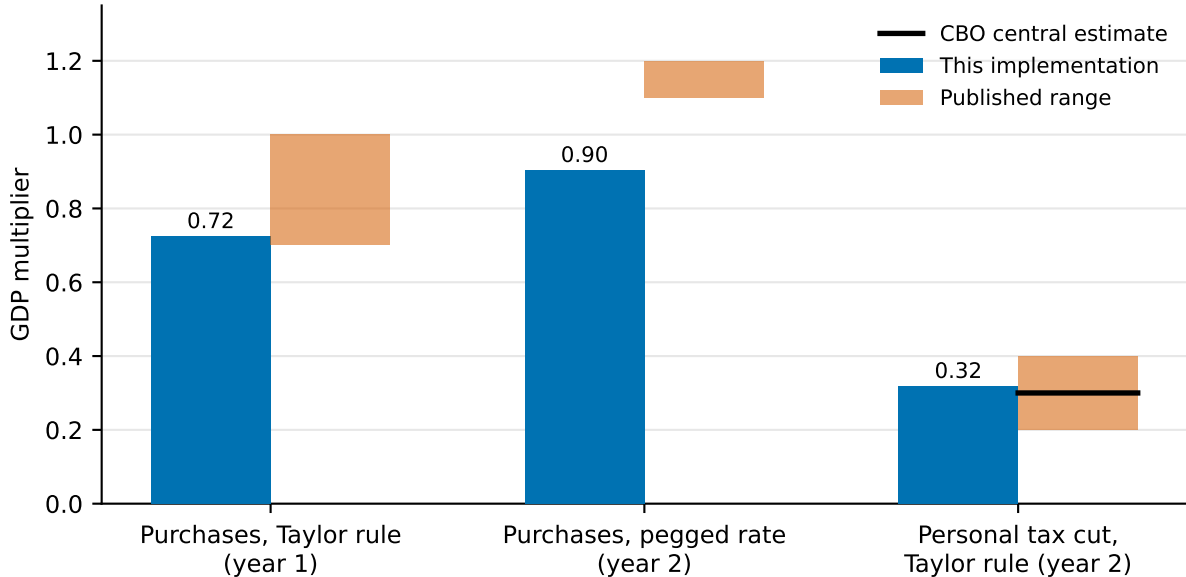
Fiscal multipliers: this implementation vs published benchmarks each bar against a band of matching horizon and monetary conditioning
