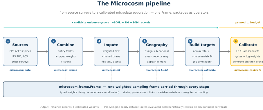
Figure 1: The two-stage pipeline. In the configuration used here, source surveys are loaded and combined into a weighted frame; stage one imputes missing variables; and stage two assigns geography, constructs administrative calibration targets, and applies target-informed L_0 selection and calibration to produce a sparse, simulable, geography-consistent release.
