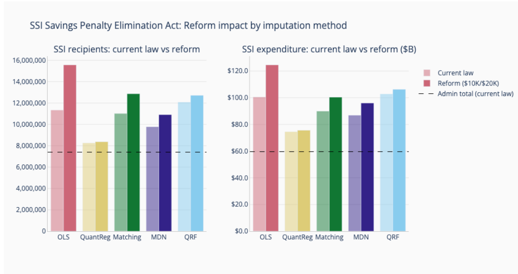
Figure 4: SSI recipients (left) and total expenditure (right) under current law (lighter bars) versus the SSI Savings Penalty Elimination Act reform (darker bars), by imputation method. The dashed line indicates the SSA administrative total under current law.
