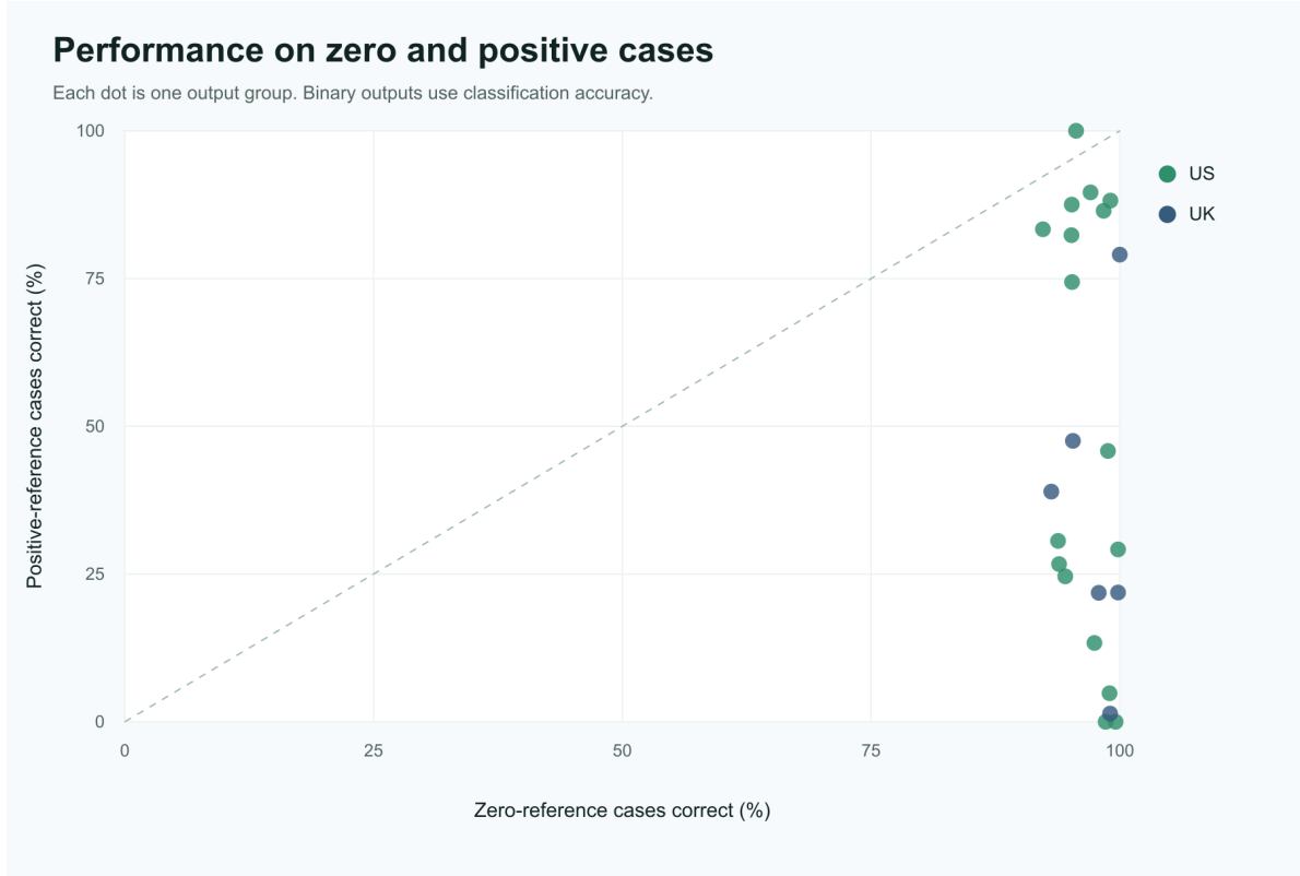
Figure 2: Output-level performance on zero-reference and positive-reference cases.
