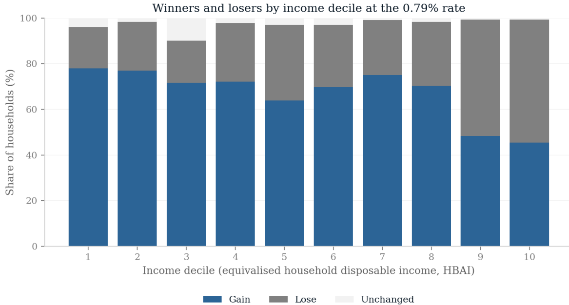
Figure 7: Share of winners and losers by income decile at the 0.79% budget-neutral rate.
