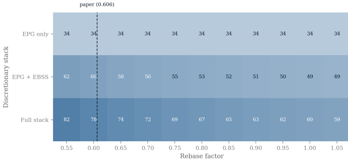
Figure 7: The two-axis sensitivity grid as a heatmap, with the rebase axis swept finely (0.55 to 1.05 in steps of 0.05; the empty stack is omitted); the dashed rule marks the paper’s computed rebase, and Table 4 reports the three canonical columns with decile detail. Cell values are the discretionary cushioning rate against the counterfactual shock. The EPG row is invariant to both axes, a price cap scales with the bill it truncates and is constant across deciles by construction, so the progressivity and the rebase-sensitivity of the headline both come entirely from the flat-cash instruments.
