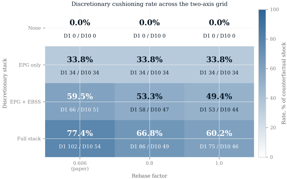
Figure 7: The two-axis grid of Table 4 as a heatmap. Cell shading is the discretionary cushioning rate against the counterfactual shock; each cell also reports the bottom- and top-decile rates. The EPG row is invariant to both axes—a price cap scales with the bill it truncates and is constant across deciles by construction—so the progressivity and the rebase-sensitivity of the headline both come entirely from the flat-cash instruments.
