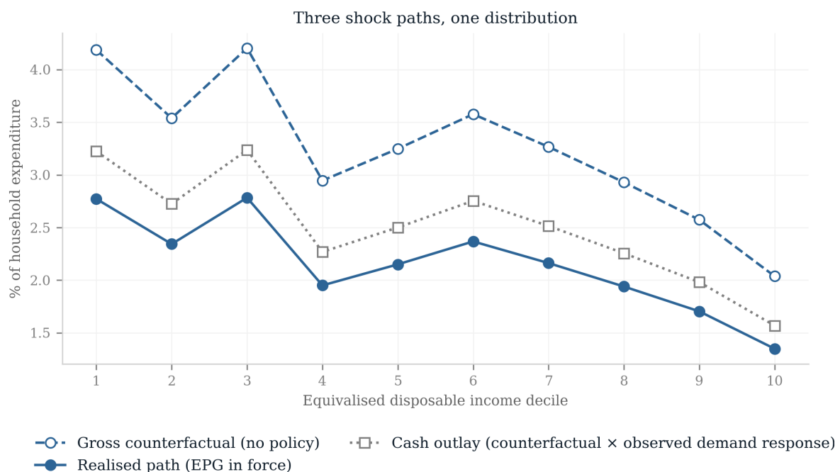
Figure 9: Three shock paths by equivalised disposable income decile, as a share of household expenditure, on the second stage's financial-year basis: the gross counterfactual (no policy), the realised path (Energy Price Guarantee in force), and the cash-outlay path (the gross counterfactual scaled by the observed weather-adjusted demand response, the first-pass convention). Level shifts, common shape.
