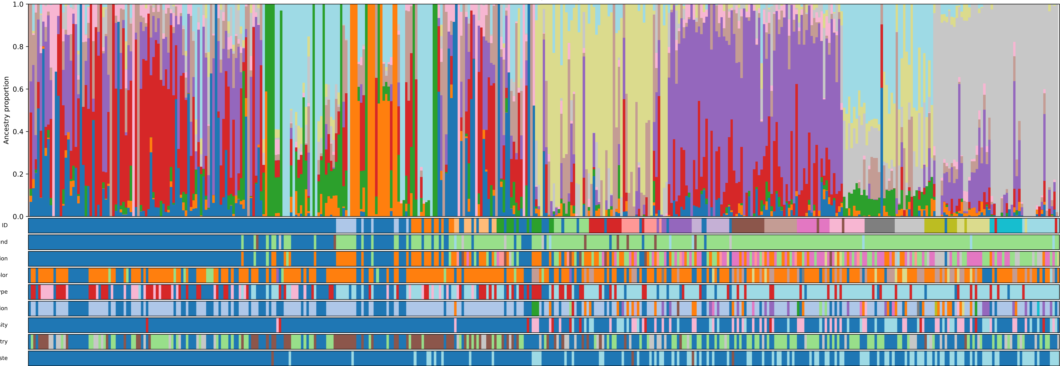
ADMIXTURE K=10
