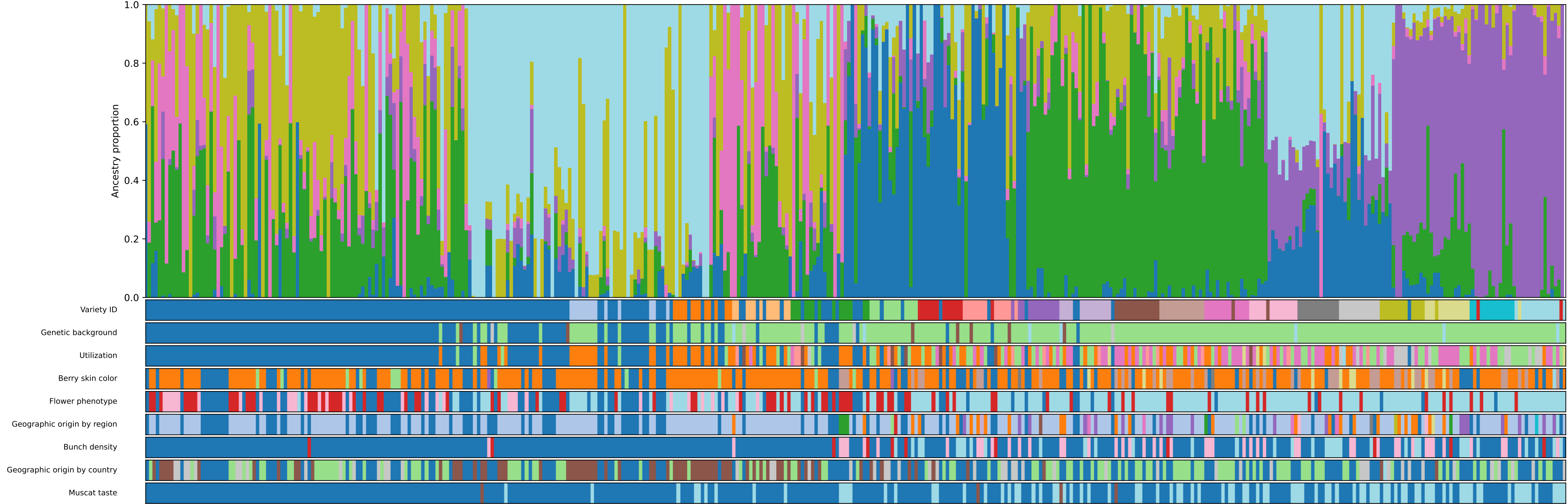
ADMIXTURE K=6
