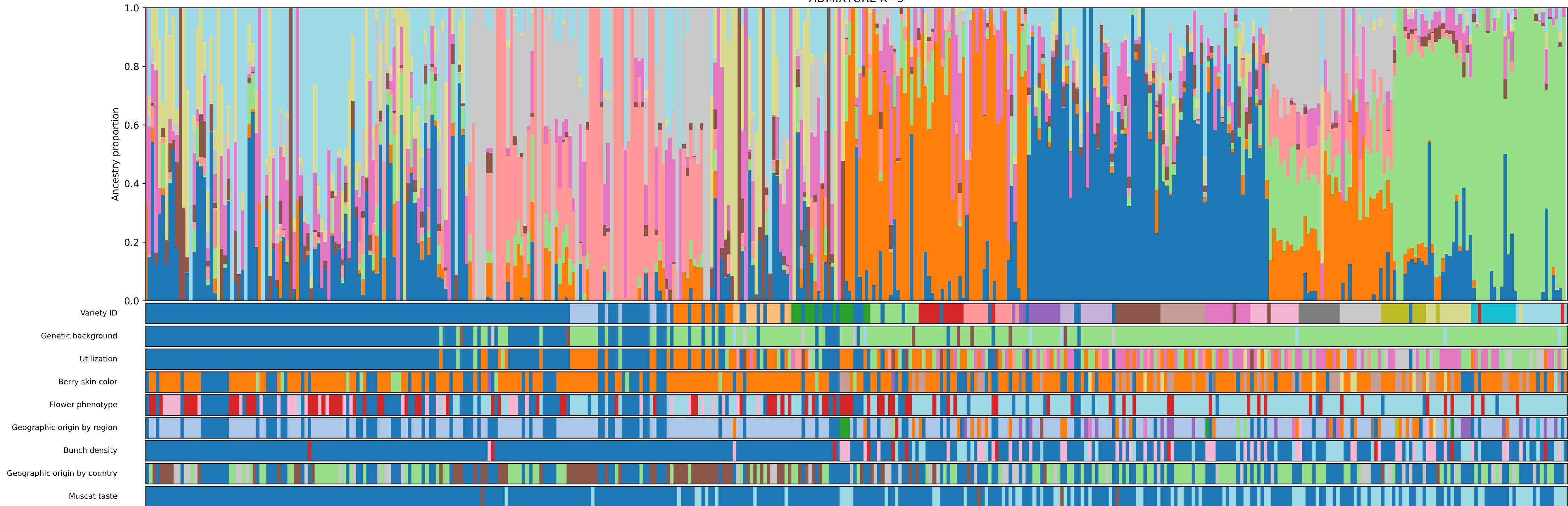
ADMIXTURE K=9
