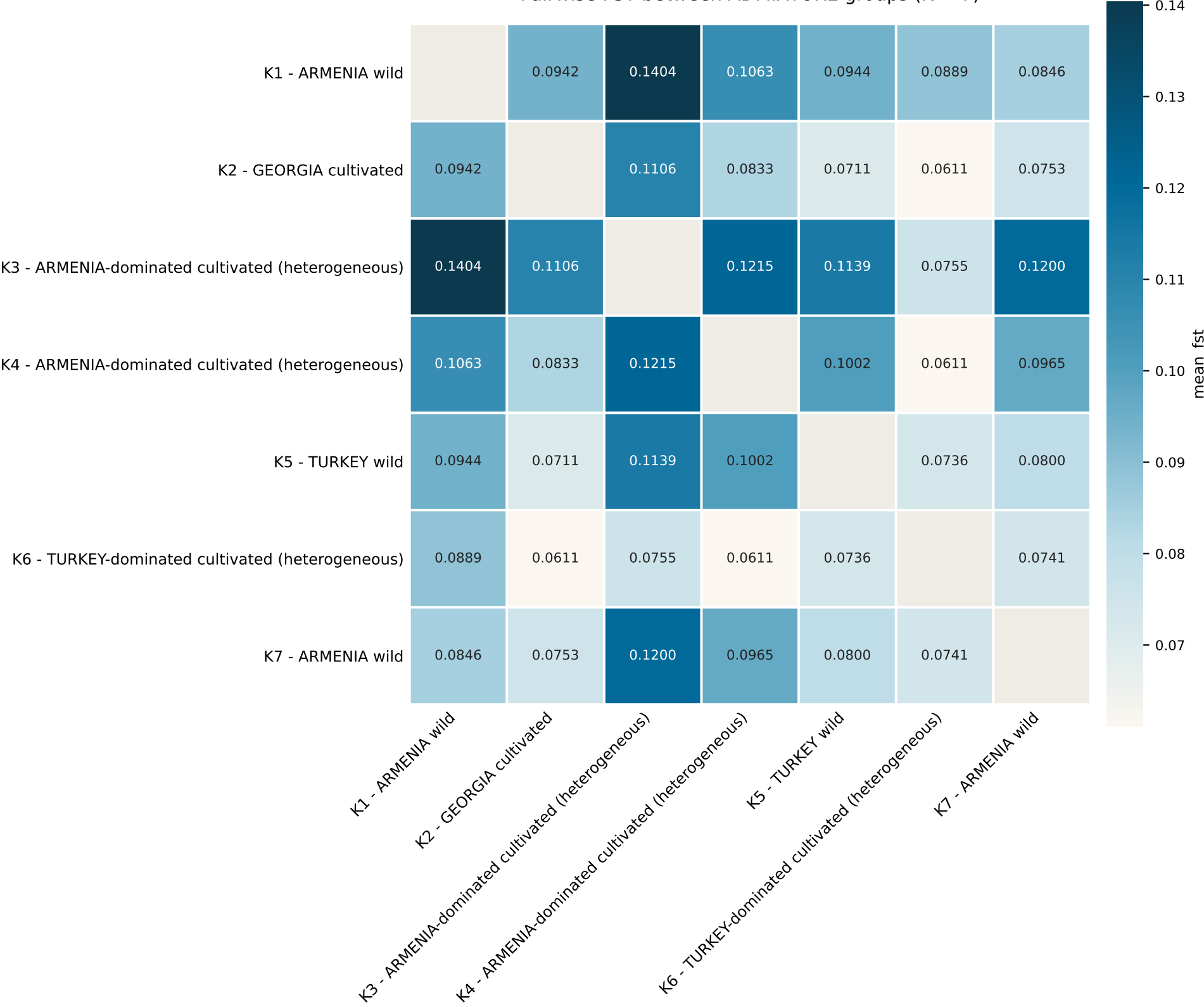
Pairwise FST between ADMIXTURE groups (K = 7)
