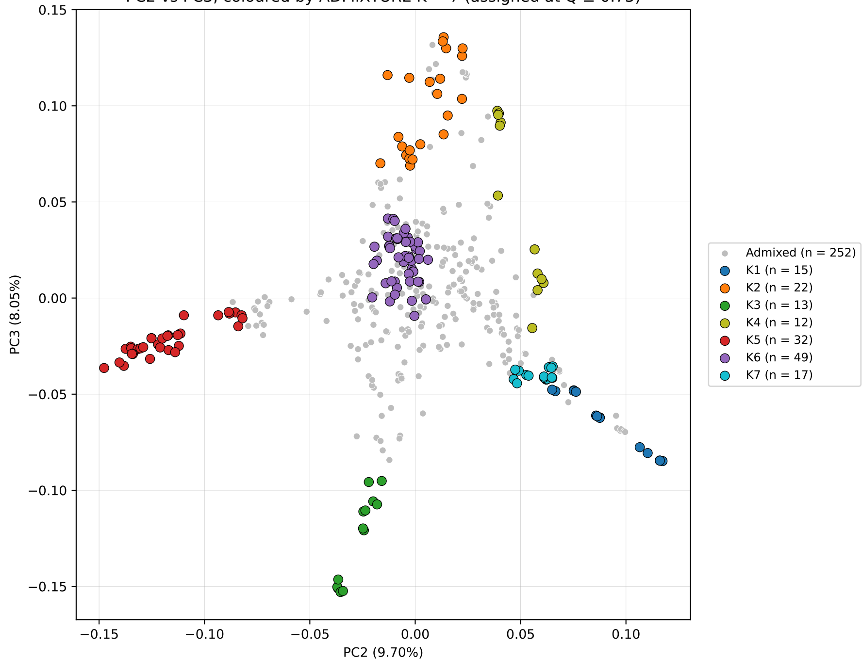
PC2 vs PC3, coloured by ADMIXTURE K = 7 (assigned at Q \geq 0.75 )
