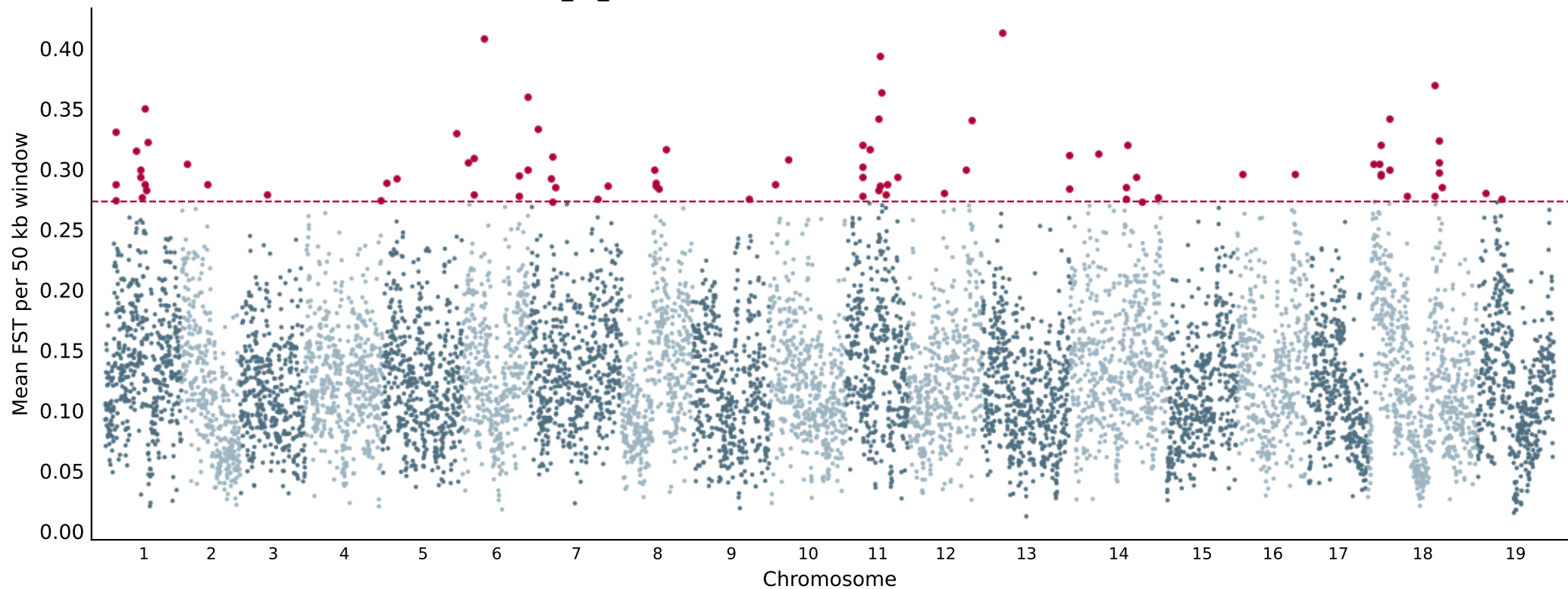
K3_vs_K7 - 8433 windows, 85 outliers above 0.2733
