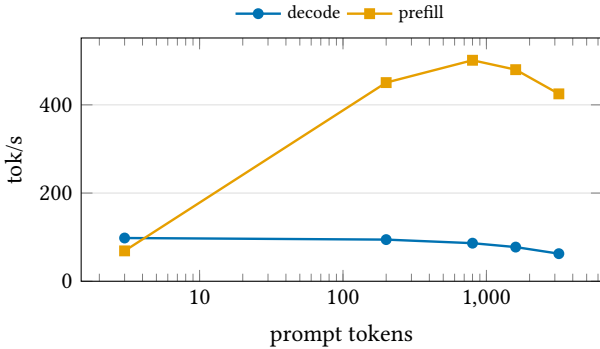
Figure 6: Context scaling (Qwen3-4B Q8_0, M5 Max Metal; error bars show MAD). Decode falls as the per-step KV read grows; prefill peaks once the matrix kernels amortize and eases as attention’s KV re-reads grow.
