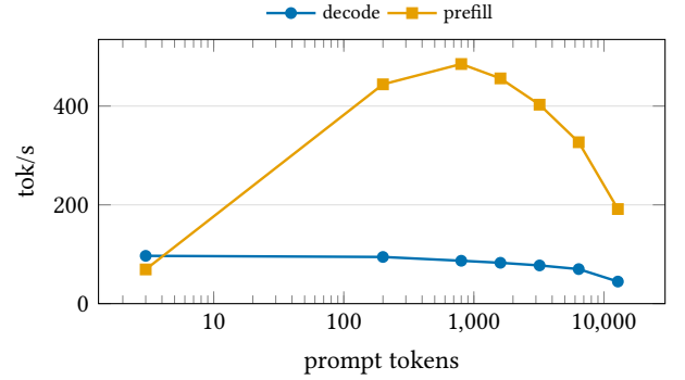
Figure 6: Context scaling (Qwen3-4B Q8_0, M5 Max Metal; error bars show MAD). Decode falls as the per-step KV read grows; prefill peaks at short context and declines as attention’s quadratic cost grows against the linear matmul work.
