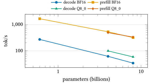
Figure 5: Throughput across the Qwen3 dense family (M5 Max Metal). Decode tracks streamed weight bytes per token; prefill tracks compute.
