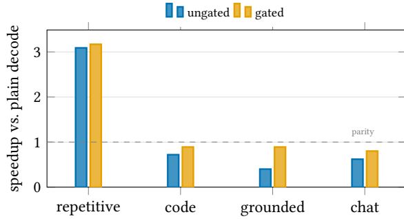
Figure 9: Speculation speedup by workload, with and without the adaptive gate. The dashed line is parity with plain decode: gating preserves the repetitive-workload win and pulls every losing workload back toward parity.
