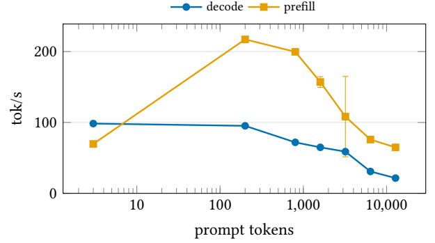
Figure 6: Context scaling (Qwen3-4B Q8_0, M5 Max Metal; error bars show MAD). Decode falls as the per-step KV read grows; prefill peaks at short context and falls as the attention-prefill kernel’s quadratic cost comes to dominate.
