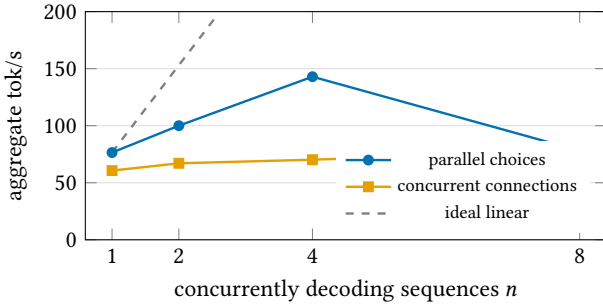
Figure 7: Batch scaling on the pooled Q8_0 server (M5 Max). The dashed line is ideal linear scaling from the single-stream rate. Scheduling overhead widens the gap, and at n=8 per-step CPU-side sampling stalls the GPU long enough for demand-scaled clocks to sag.
