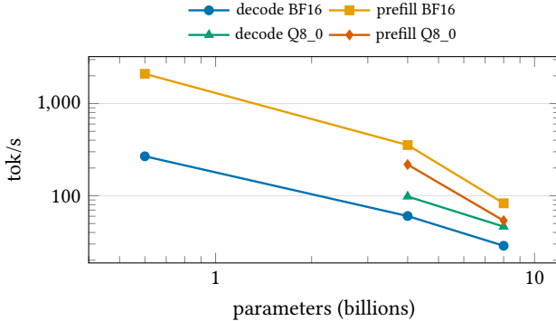
Figure 5: Throughput across the Qwen3 dense family (M5 Max Metal). Decode tracks streamed weight bytes per token; prefill tracks shared compute.
