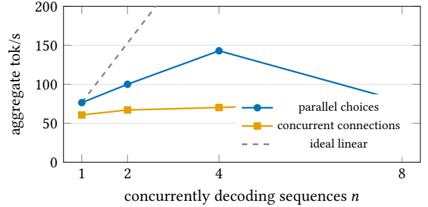
Figure 7: Batch scaling on the pooled Q8_0 server (M5 Max). The dashed line is ideal linear scaling from the single-stream rate. Scheduling overhead widens the gap, and at n=8 per-step CPU-side sampling stalls the GPU long enough for demand-scaled clocks to sag.
