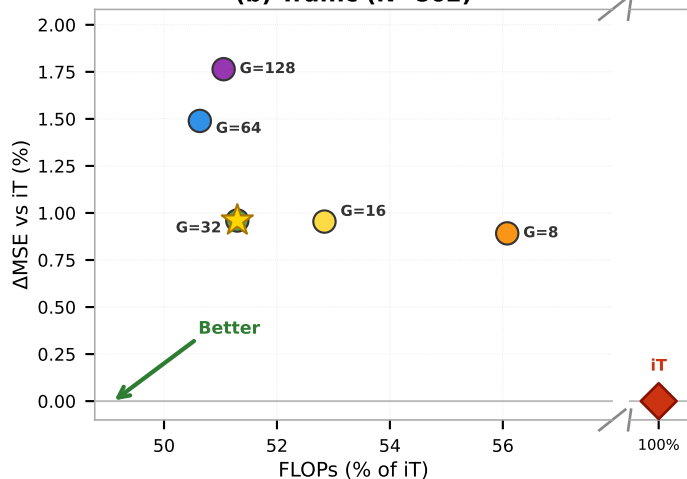
(b) Traffic (N=862)
