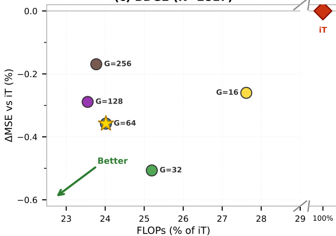
(c) BDG2 (N=2817)
