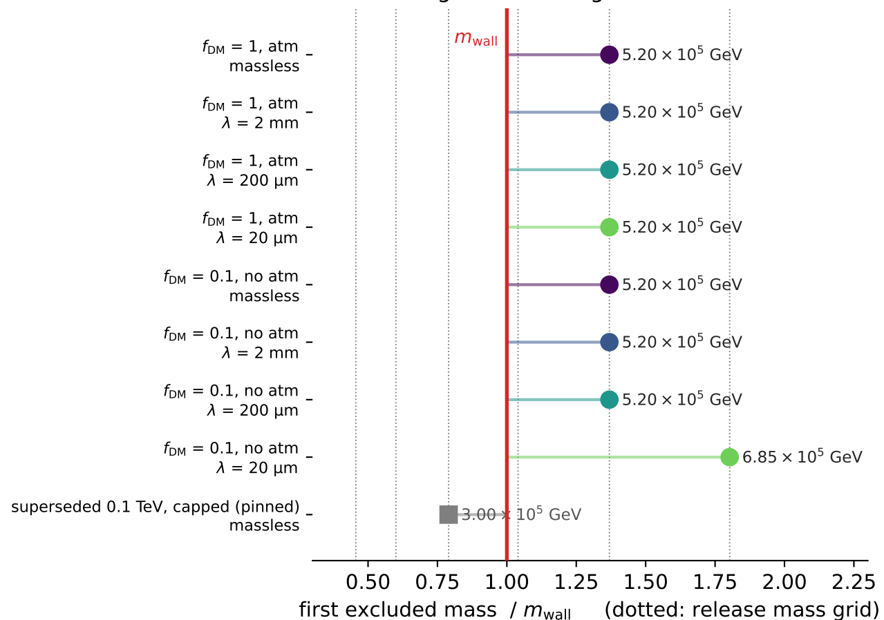
B. Each edge is the first grid mass above the wall
