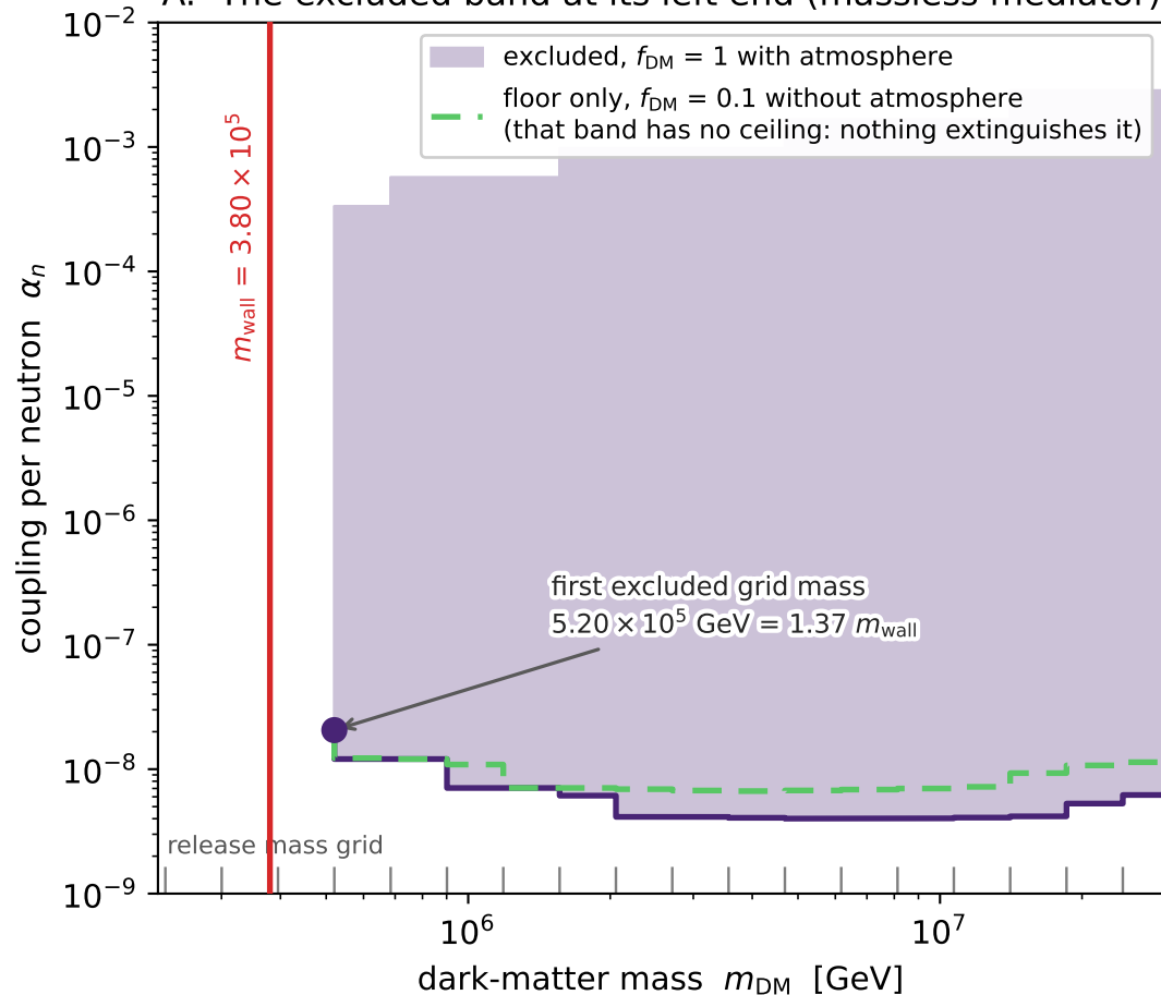
A. The excluded band at its left end (massless mediator)
