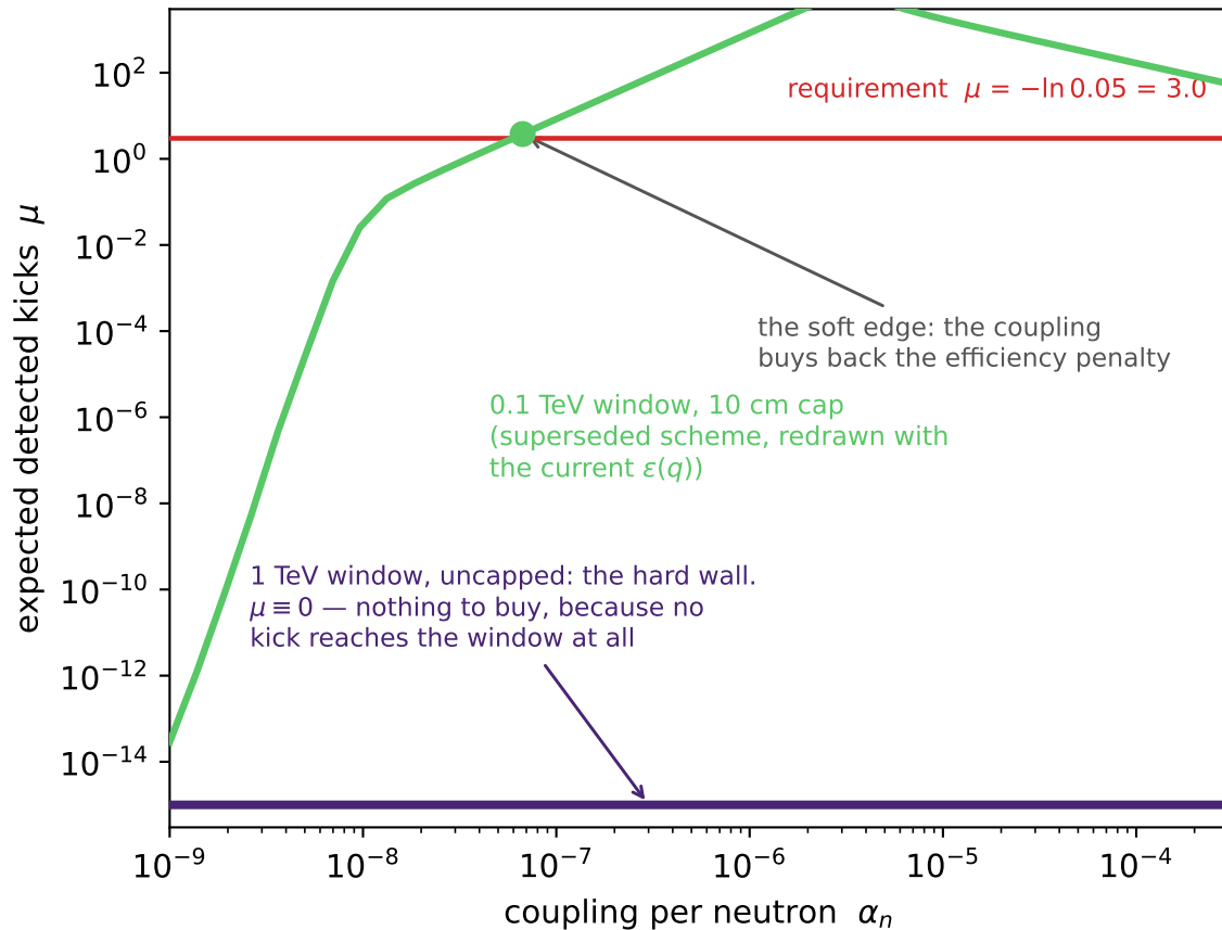
B. At m_{\text{DM}} = 3.00 \times 10^5 GeV ( = 0.79 m_{\text{wall}} )
