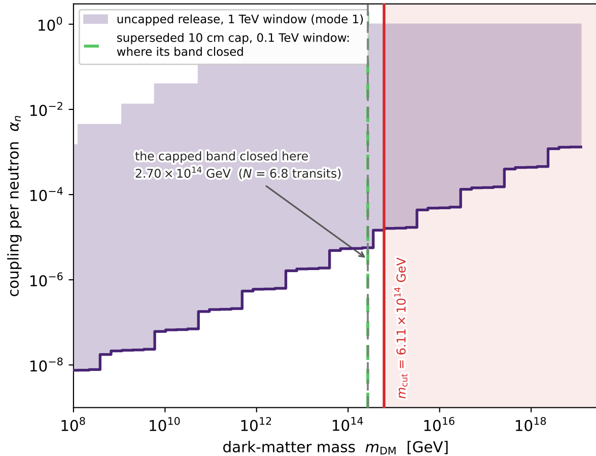
A. Two ways to stop: cap the integral, or cut in mass
