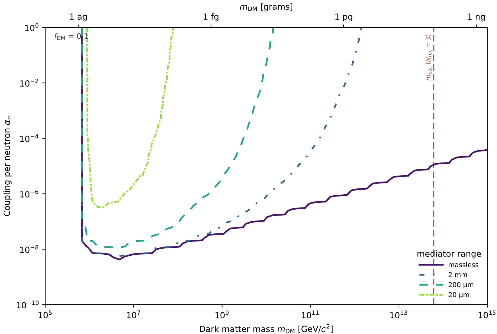
Three-mode 95% CL exclusion, no atmosphere, q_{\min} = 1 TeV
