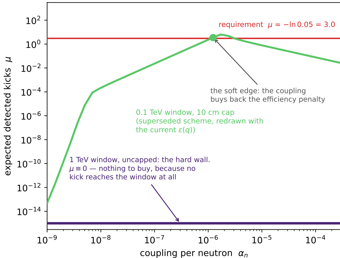
B. At m_{\text{DM}} = 3.00 \times 10^5 GeV ( = 0.54 m_{\text{wall}} )
