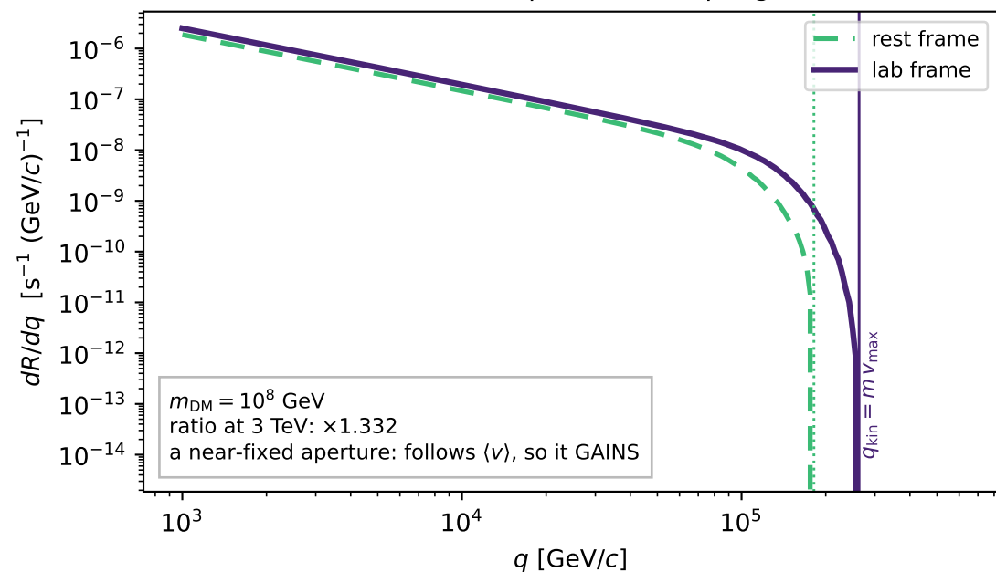
D. \lambda = 200 \mu\text{m} , bulk coupling
