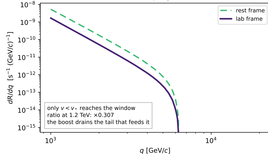
C. Massless, near the coupling floor ( \alpha_n = 2.5 \times 10^{-9} )
