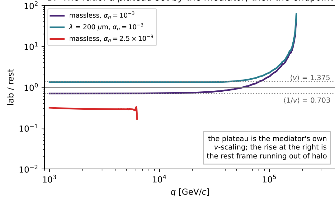
D. \lambda = 200 \mu\text{m} , bulk coupling
