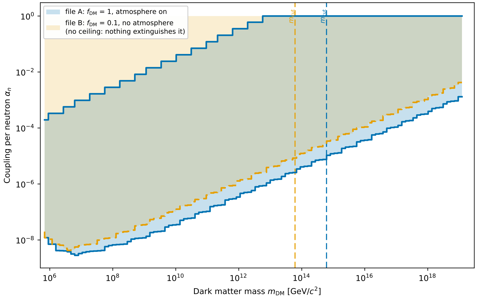
The two released hypotheses (mode 1, massless mediator): they differ in both f_{\text{DM}} and atmosphere
