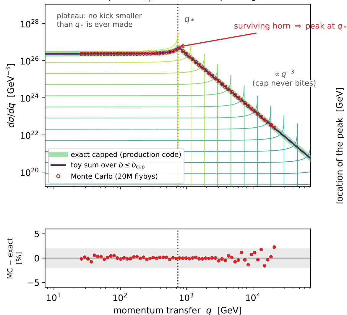
C. Cap b \leq b_{\text{cap}} : kicks below q_* are gone
