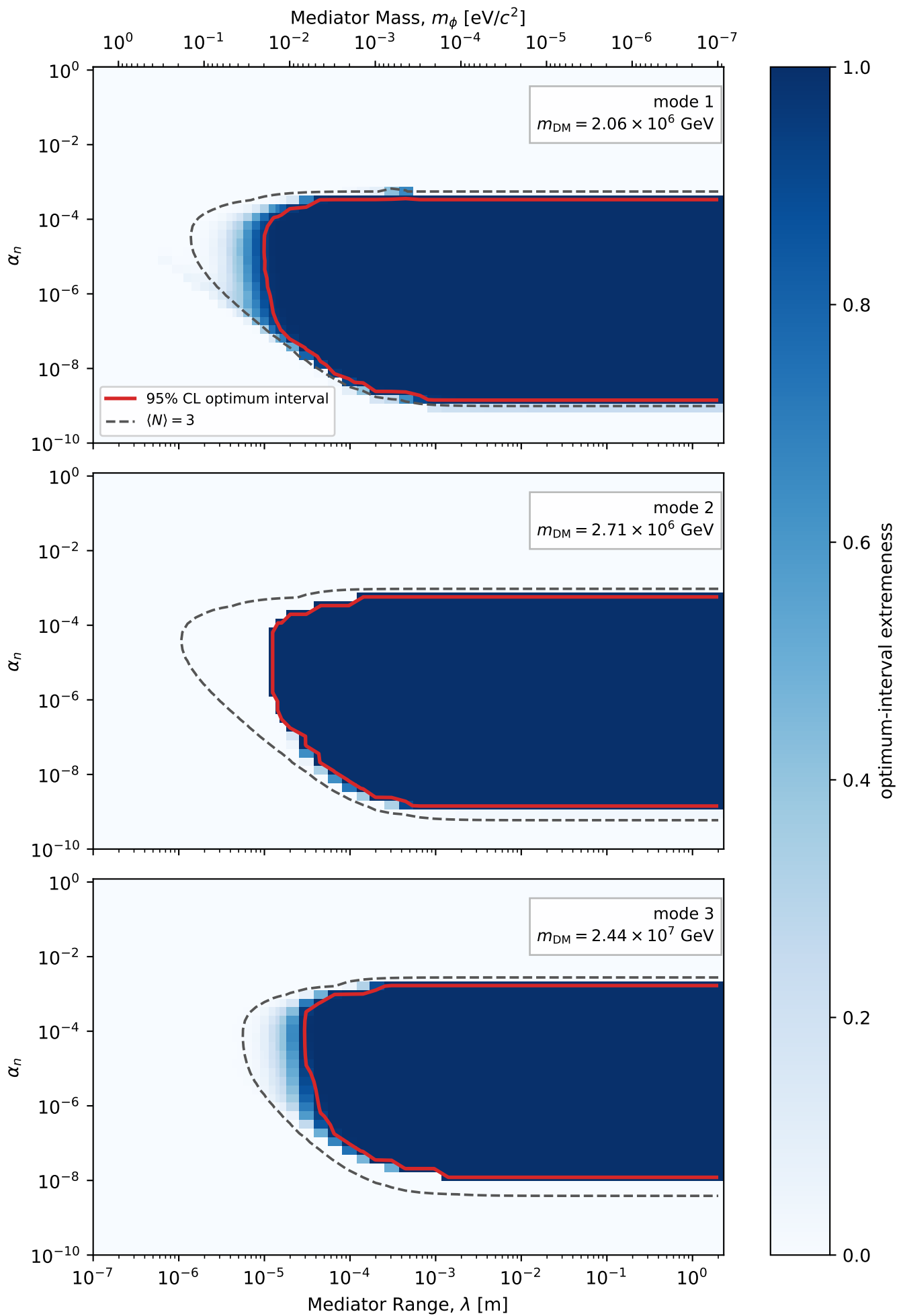
Mediator range vs coupling, per mode ( \lambda : 0.1 \mu\text{m} - 2 m)
