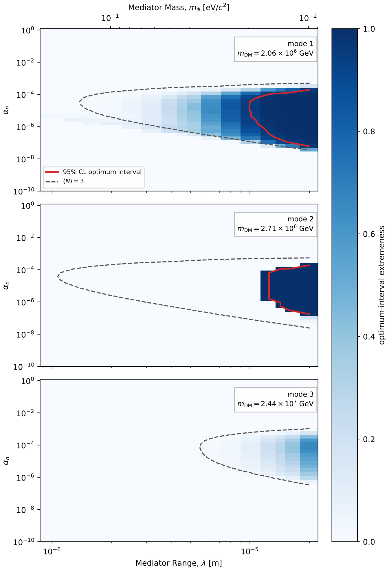
Mediator range vs coupling, per mode (zoom: 1–20 \mu\text{m} )
