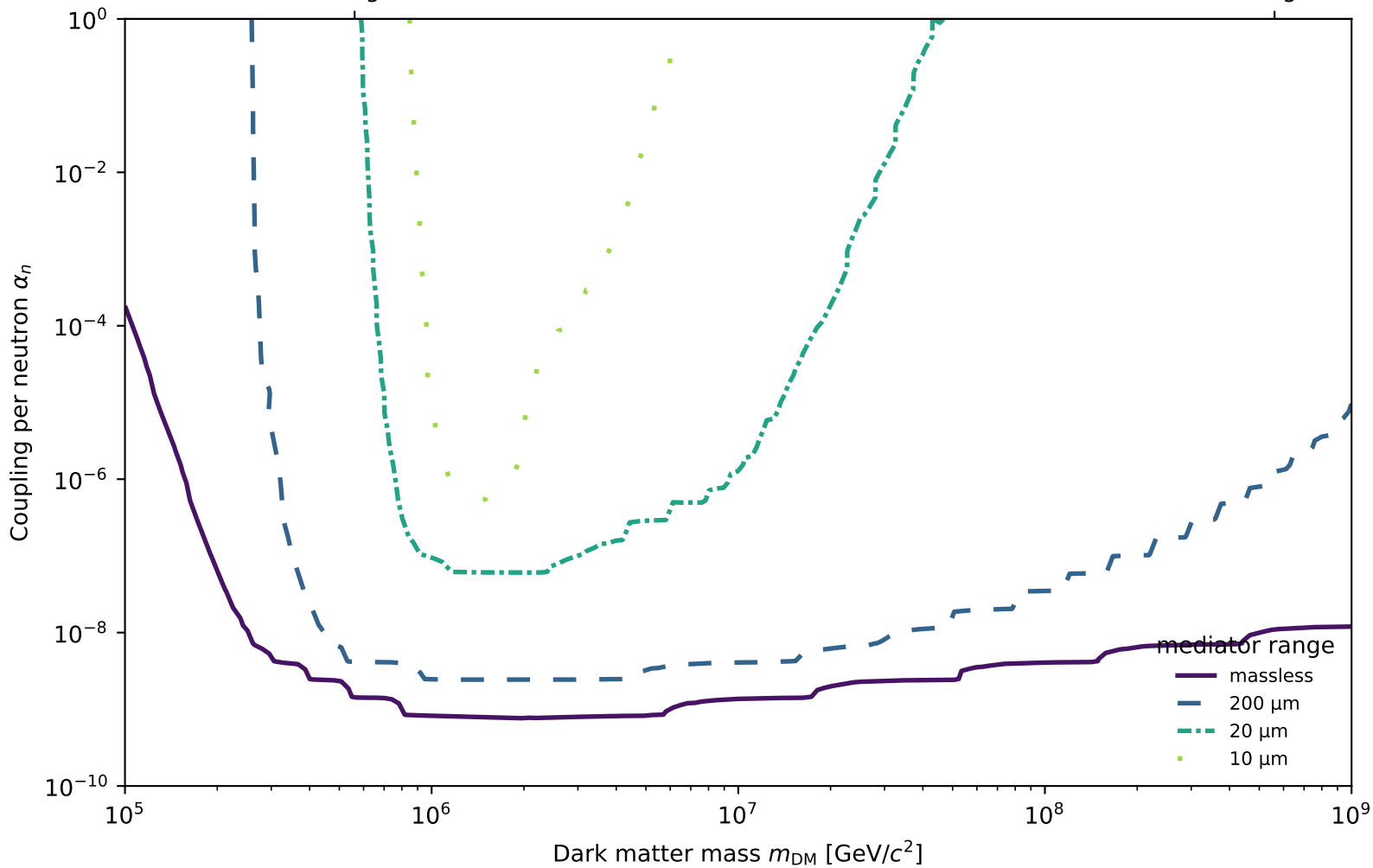
Composite (3-mode) 95% CL exclusion, no atmosphere, q_{\min} = 0.1 TeV
