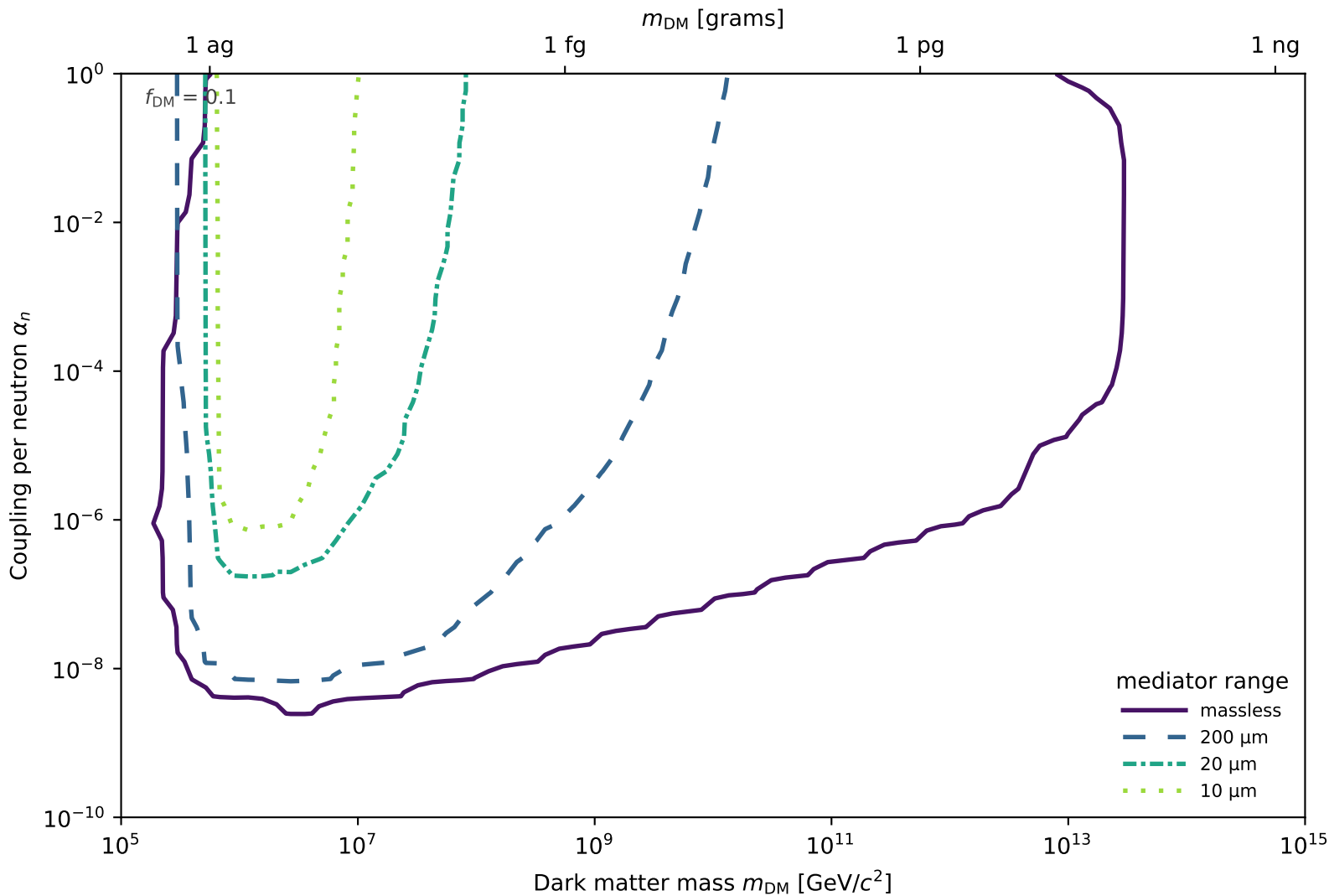
Three-mode 95% CL exclusion, no atmosphere, q_{\min} = 0.1 TeV
