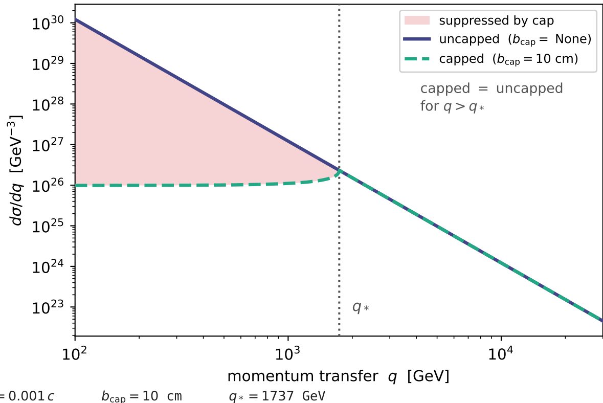
B. Effect on d\sigma/dq
