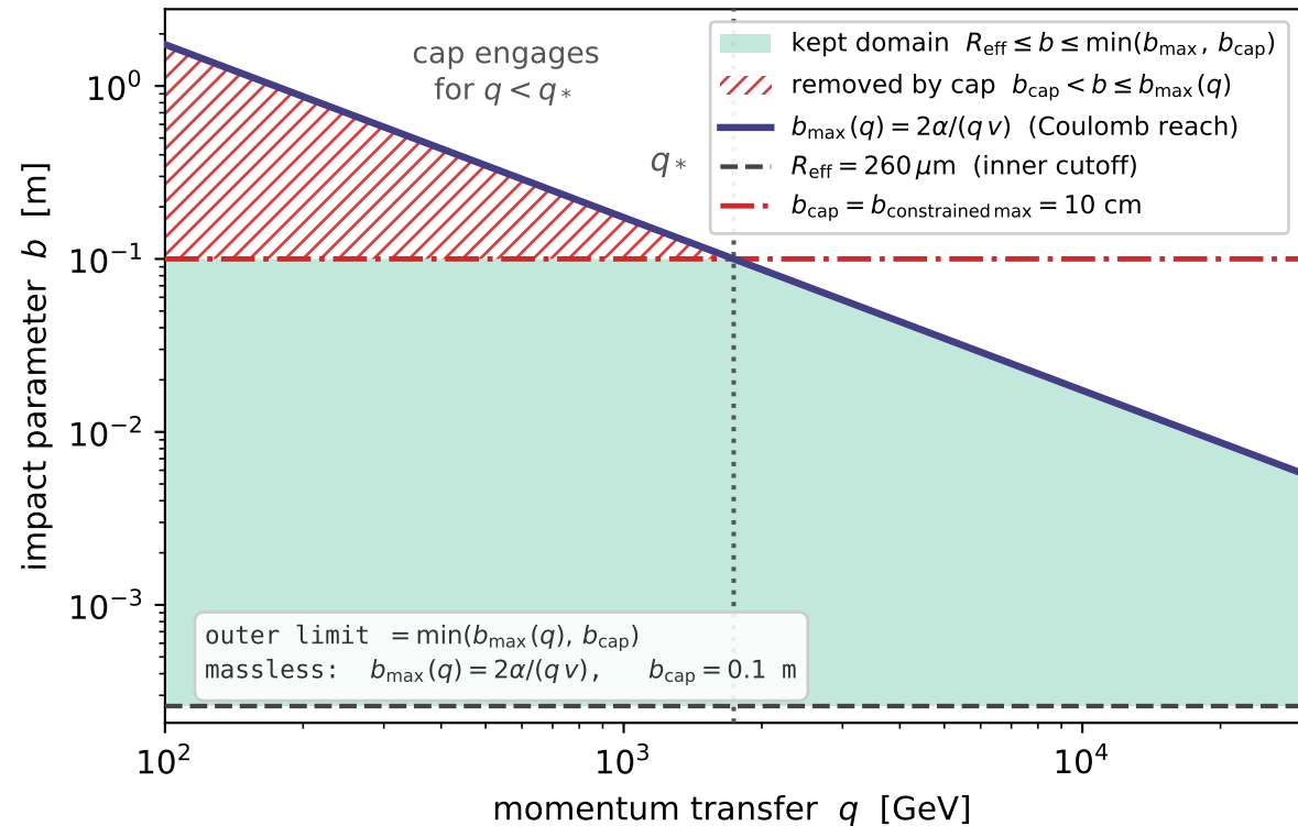
A. Integration domain in the (q, b) plane
