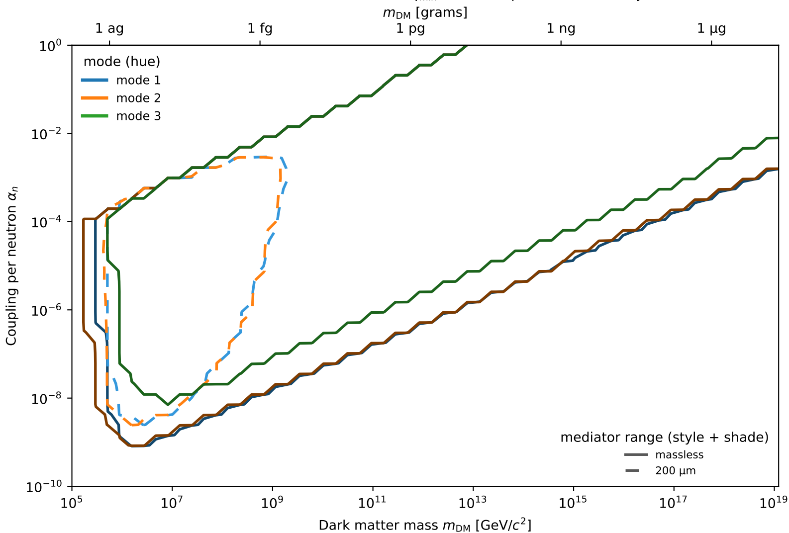
95% CL exclusion (all modes), q_{\min} = 0.1 TeV, per-mode efficiency
