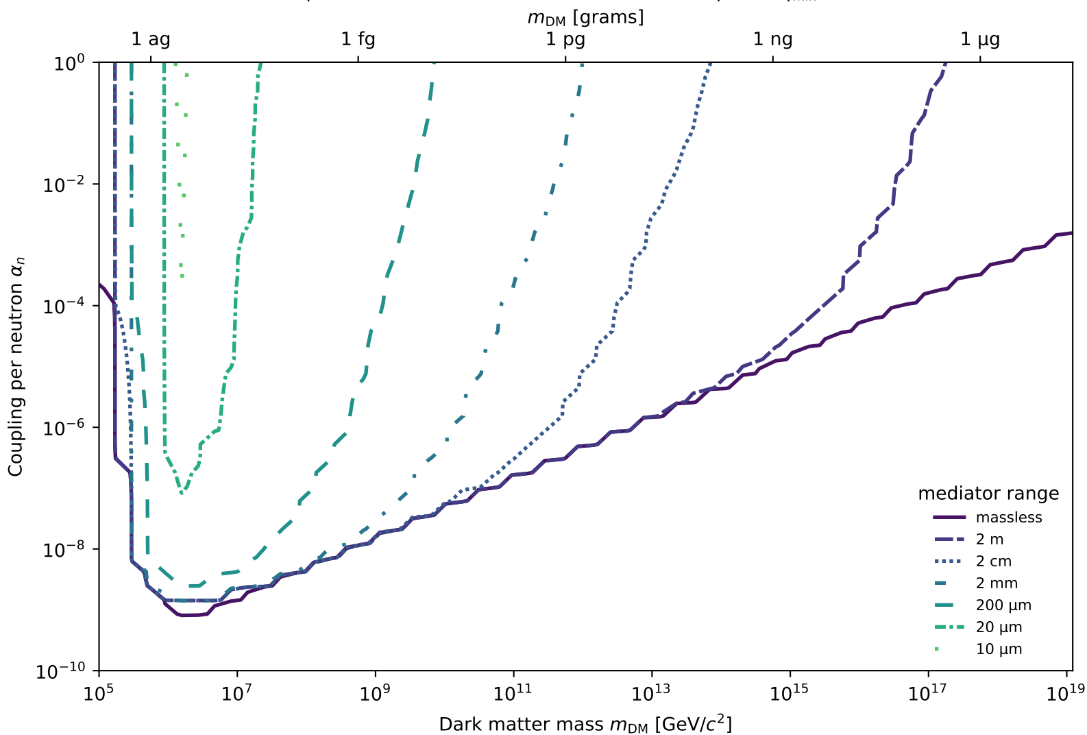
Composite (3-mode) 95% CL exclusion, no atmosphere, q_{\min} = 0.1 TeV
