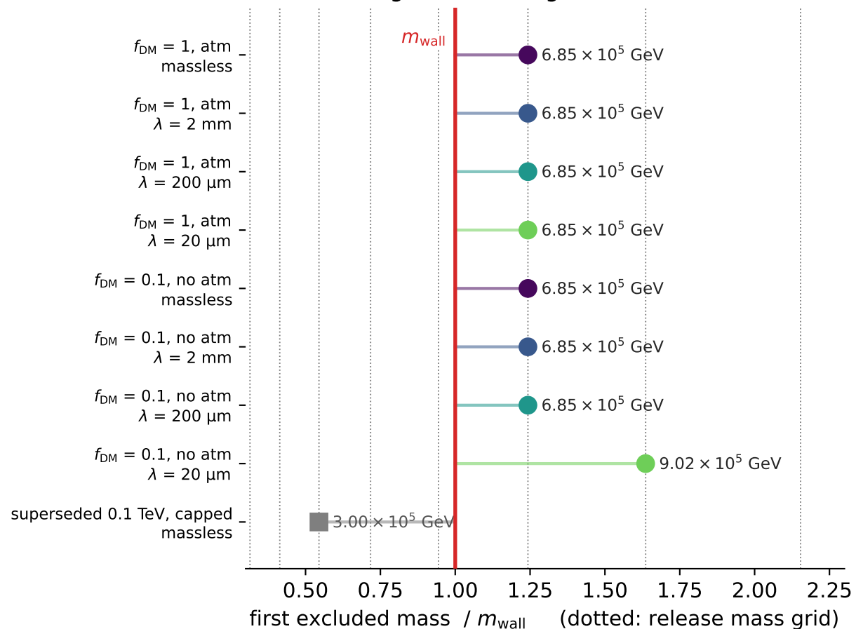
B. Each edge is the first grid mass above the wall
