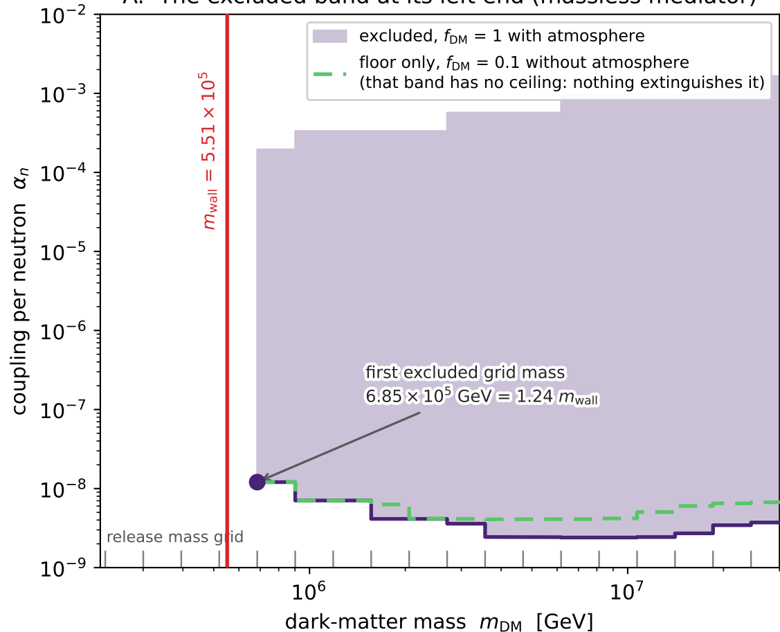
A. The excluded band at its left end (massless mediator)
