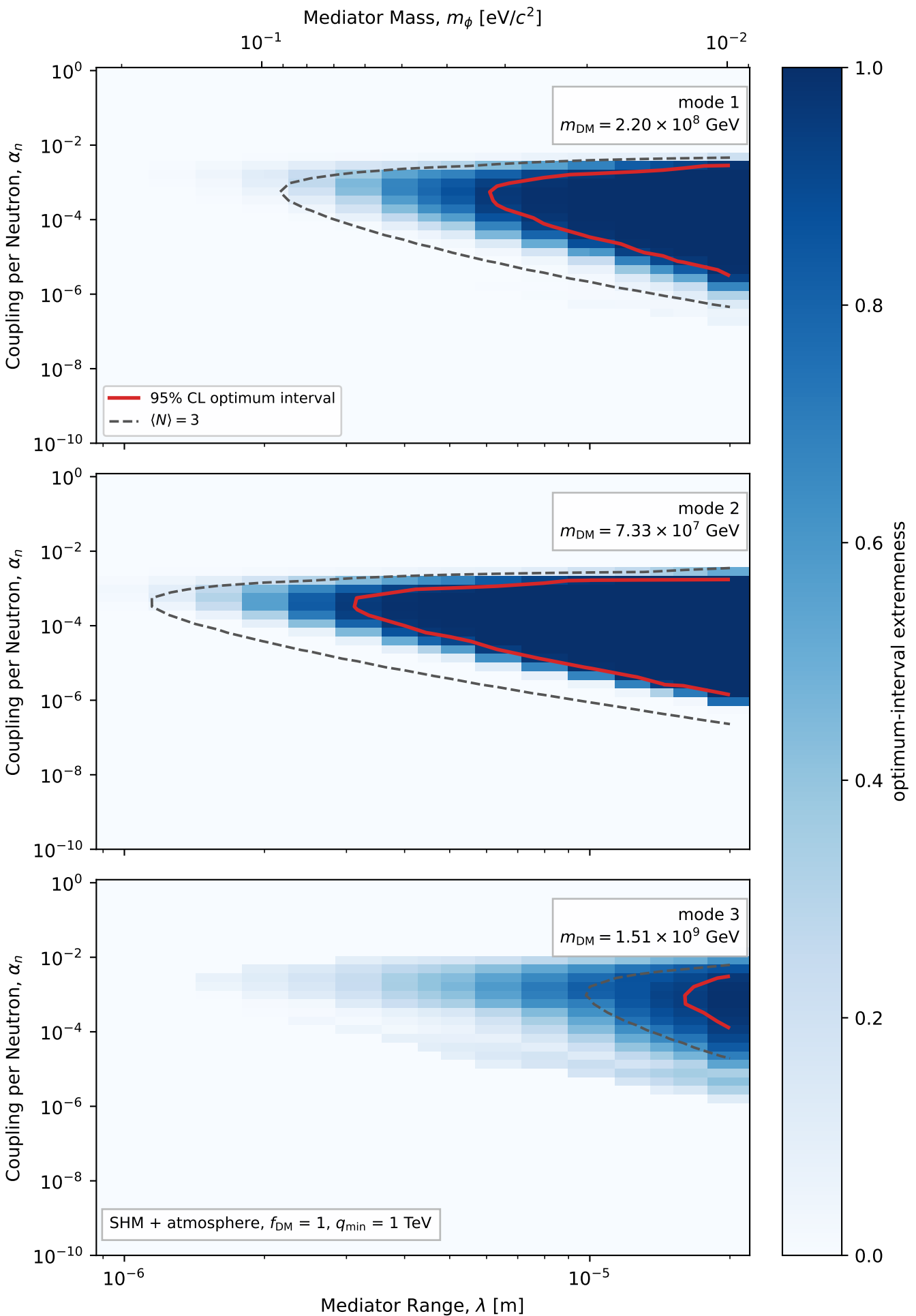
Mediator range vs coupling, per mode (zoom: 1–20 \mu\text{m} )
