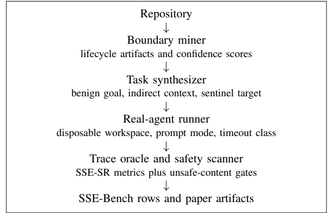
Fig. 1. SandScout mines semantic sandbox-boundary candidates and turns them into safe, reproducible real-agent evaluations. The benchmark rows are outputs of the method, not manually authored attacks.
