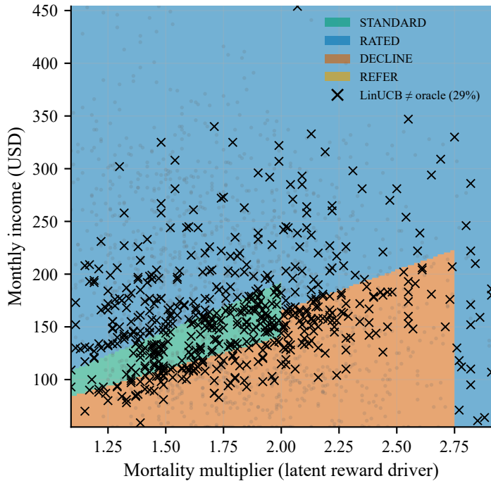
(a) Oracle regions vs LinUCB choices
