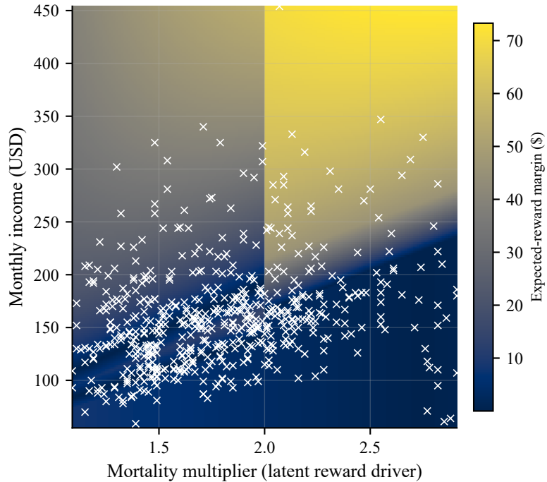
(b) Decision margin (best – 2nd-best)
