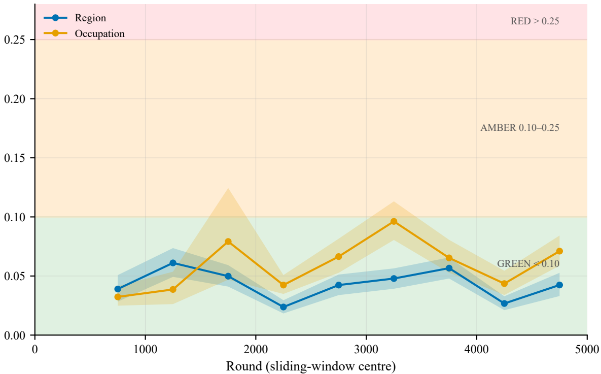
Sliding-window PSI vs reference window
