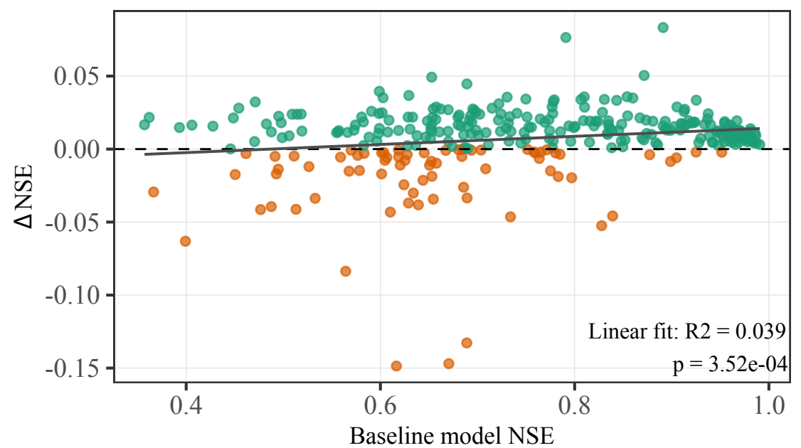
(e) NSE improvement relative to baseline performance
