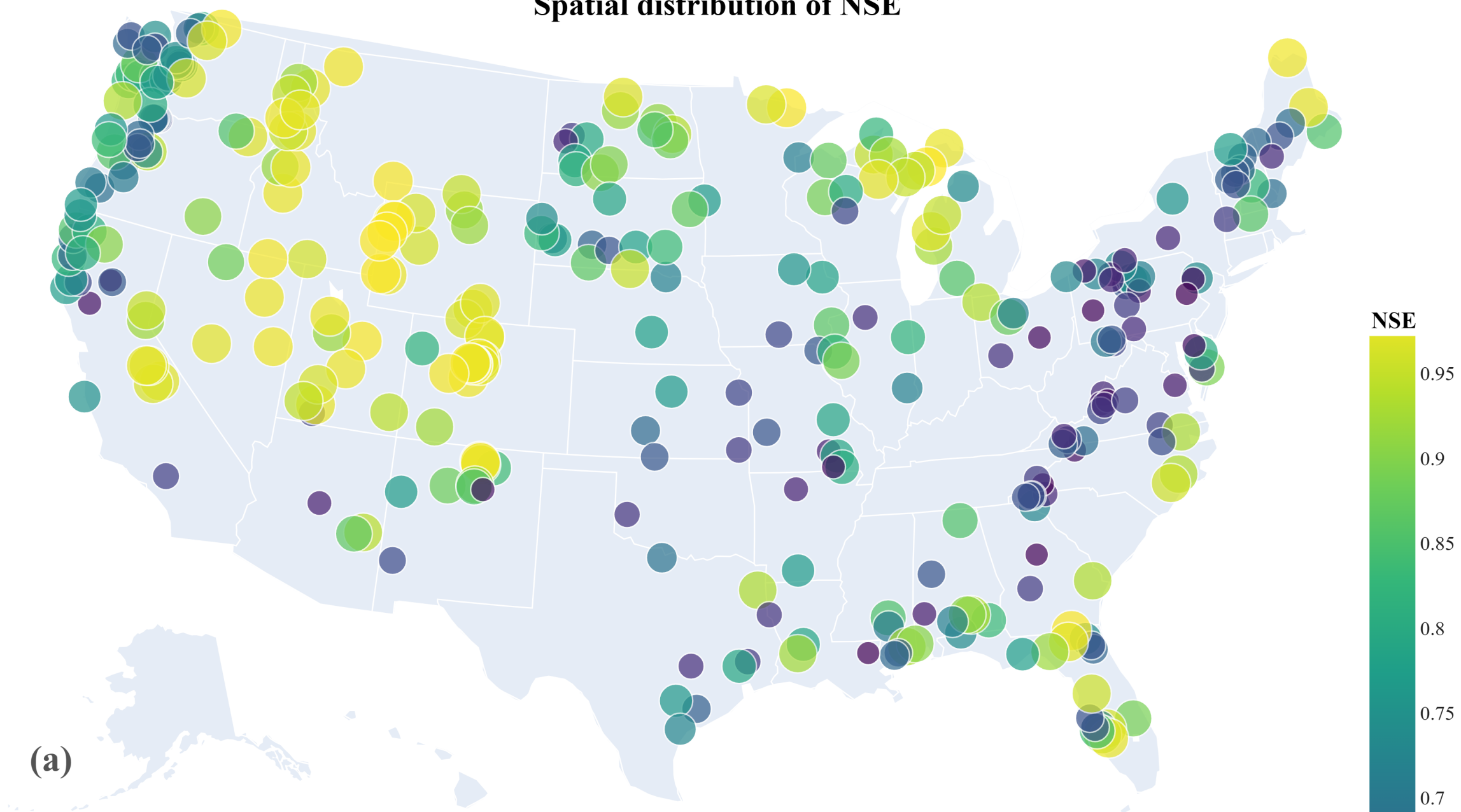
NSE Distribution
