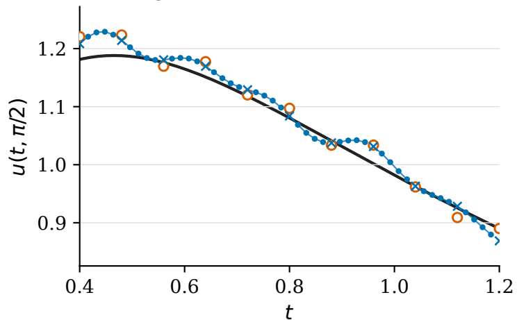
(b) Burgers: POD-EDMD-RBF
