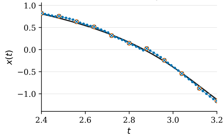
(a) Van der Pol: EDMD-polynomial
