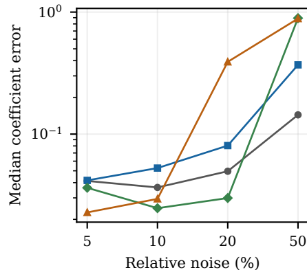
Fisher-KPP
