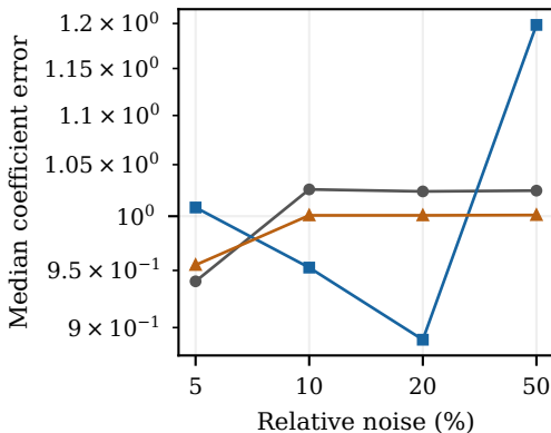
Fisher-KPP
