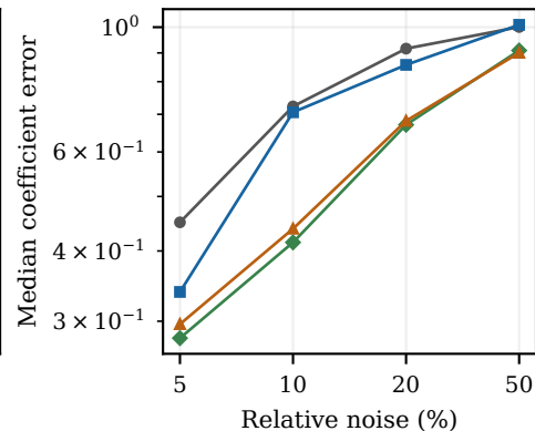
Burgers
