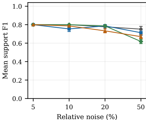
Fisher-KPP
