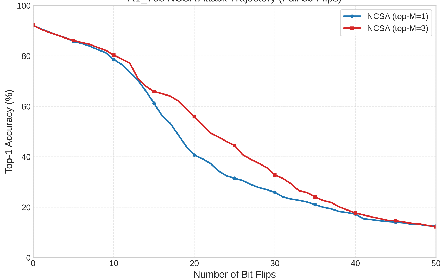
R1_T08 NCSA Attack Trajectory (Full 50 Flips)
