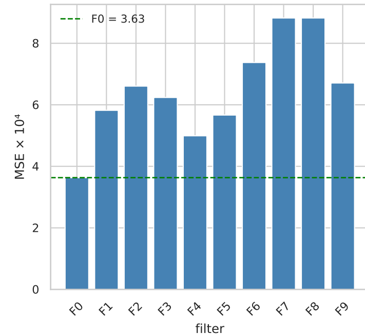
(b) Real-data: holdout MSE (Adam) — filtering hurts
