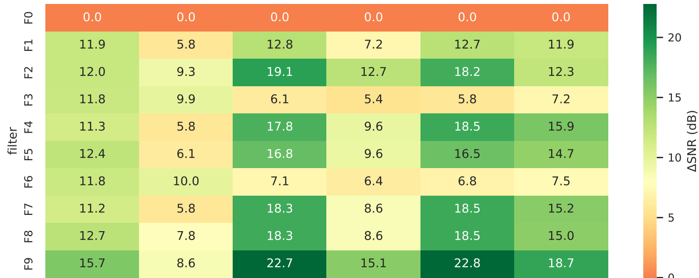
(a) Synthetic SNR gain: F0-F9 × N1-N6 (10 seeds, T=4096)
