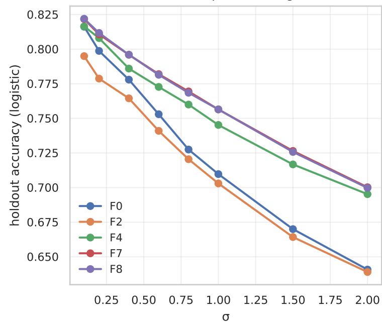
(c) \sigma -scan on \alpha -stable noise — filters help more at high \sigma
