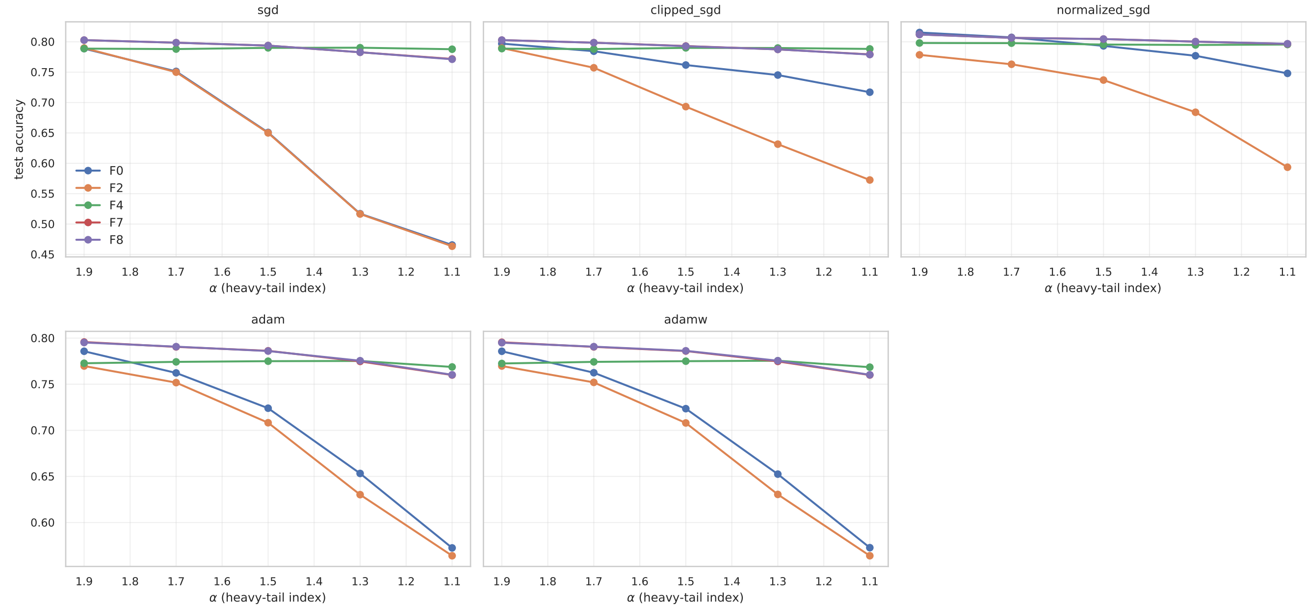
Stress test: holdout accuracy vs heavy-tail index \alpha (lower \alpha = heavier tails)
